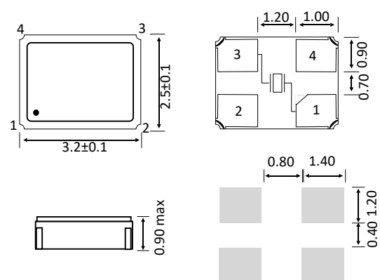
Dimensions (mm)
