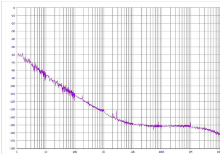
Typical Phase Noise C31-026.0M
